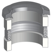
Telescopic Seal Kits
